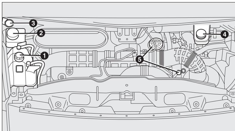
fig. 216 – Versions 115 Multijet
